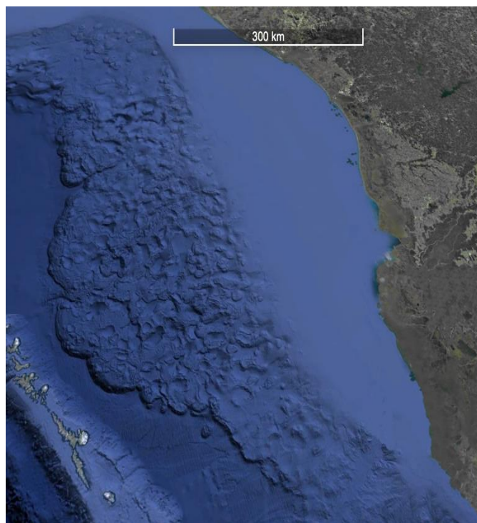
Figure 2. Possible analog of the paleogeography of Peru at some time during the mid-Jurassic to mid-Cretaceous interval, largely inspired by the present-day features of the northern Gulf of Mexico (this comparison is obviously valid only for the coeval backarc region of Peru). The idea of a salt canopy moving downslope, as illustrated by the image, is part of the analogy (ongoing research).
